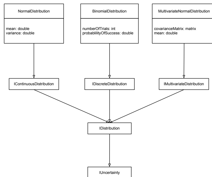
Figure 4: A selection of the distributions in UncertML represented as a UML model.
