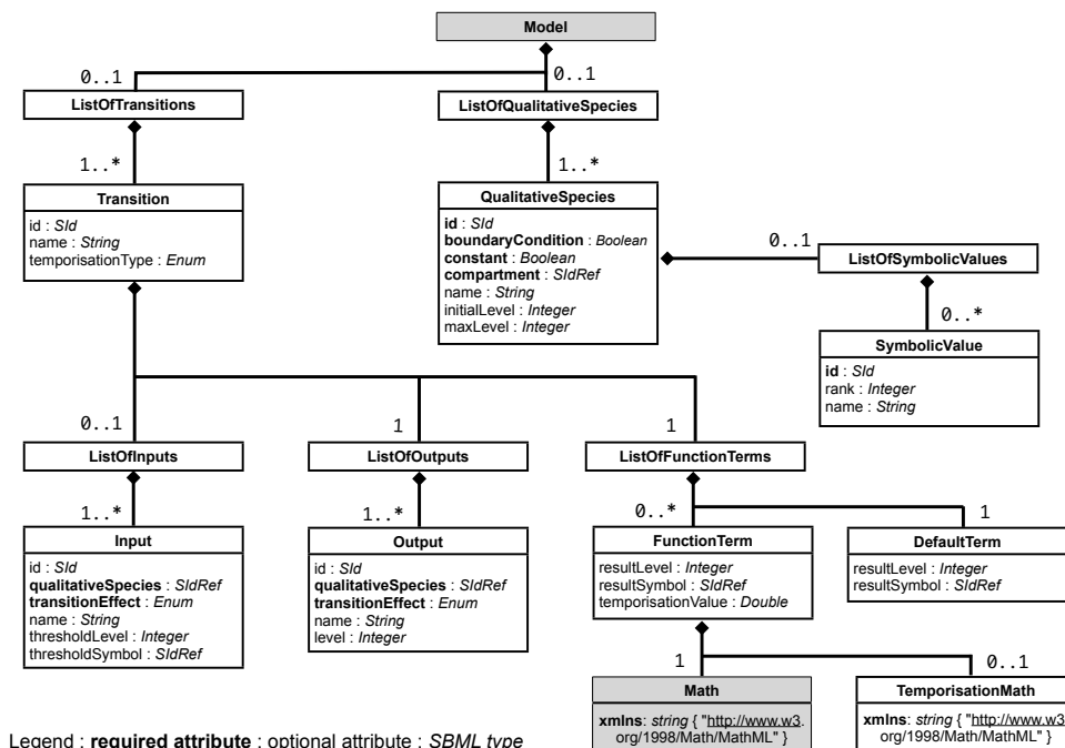
Figure 1: UML diagram of the proposal of Qualitative Models package for SBML Level 3
