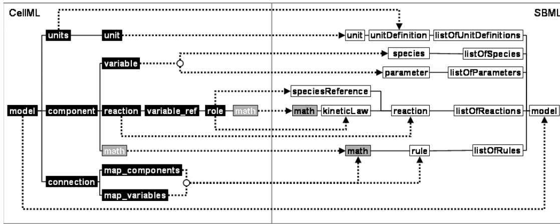
Fig. 1. Class structure of CellML (black boxes) and SBML (white boxes), and their MathML elements (gray boxes). The CellML import and group , and the SBML compartment and event elements have been omitted (see text). Solid lines indicate encapsulation (a CellML element is encapsulated by the elements on its left; the SBML elements by the one on its right). Dashed arrows indicate how the CellML elements translate into their corresponding SBML elements.
