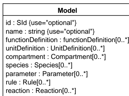
Figure 4: The definition of Model . Additional fields are inherited from SBase .
